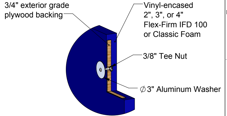
DETAIL A SCALE 1 : 8
