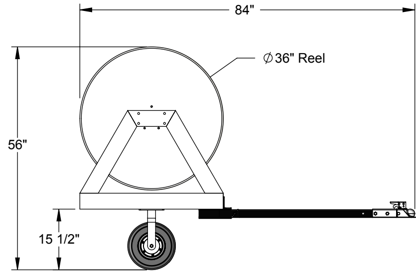
Hitch Attachment - Tow Position
