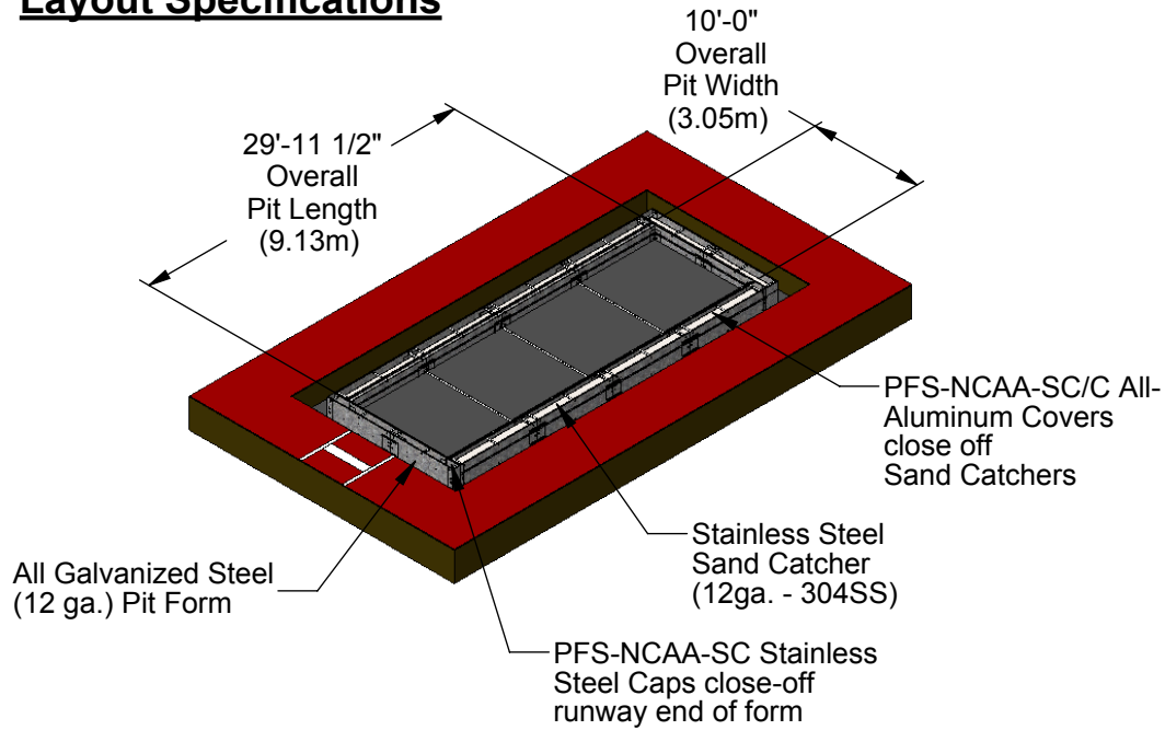
Isometric View
